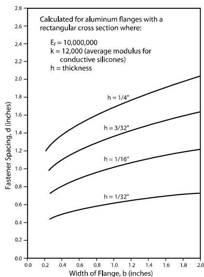
Figure 1-13. Fastener Spacing
