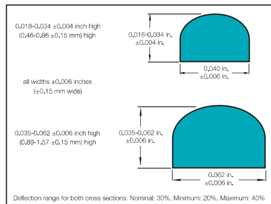
Figure 7-4 Suggested cross sections with height-to-width ratio of 0.85
