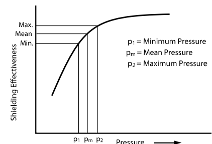
Figure 1-15. Typical Gasket Performance Curve
