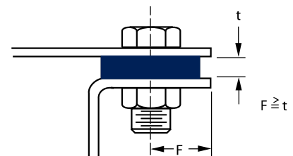
Figure 1-4. Flat Gasket on Sheet Metal Flange
