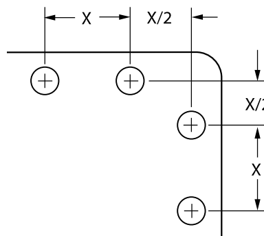
Figure 1-8. Fastener Location Near Corners
