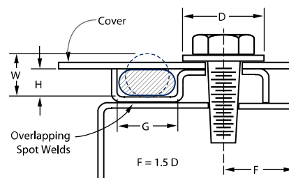
Figure 1-2. Shaped Sheet Metal Container
